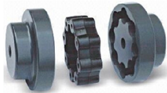
MH COUPLING
